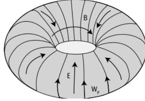
Figure 2. Schematic field geometry of the stationary electromagnetic torus.
